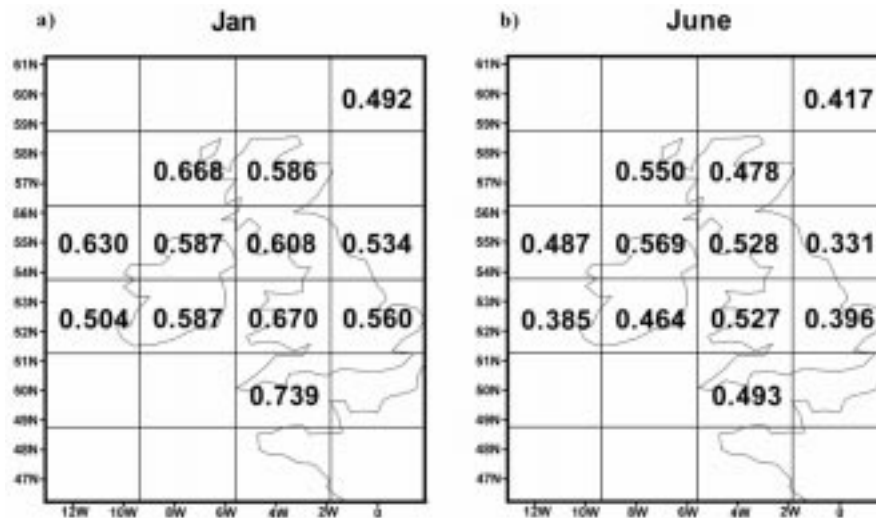
Figure 4. Variance ( R^2 ) in (a) January and (b) June gridded U.K. and Ireland precipitation explained by 1–3 indices of concurrent North Atlantic SLP using a simple stepwise linear regression model (as outlines in Murphy and Washington, 2000).
